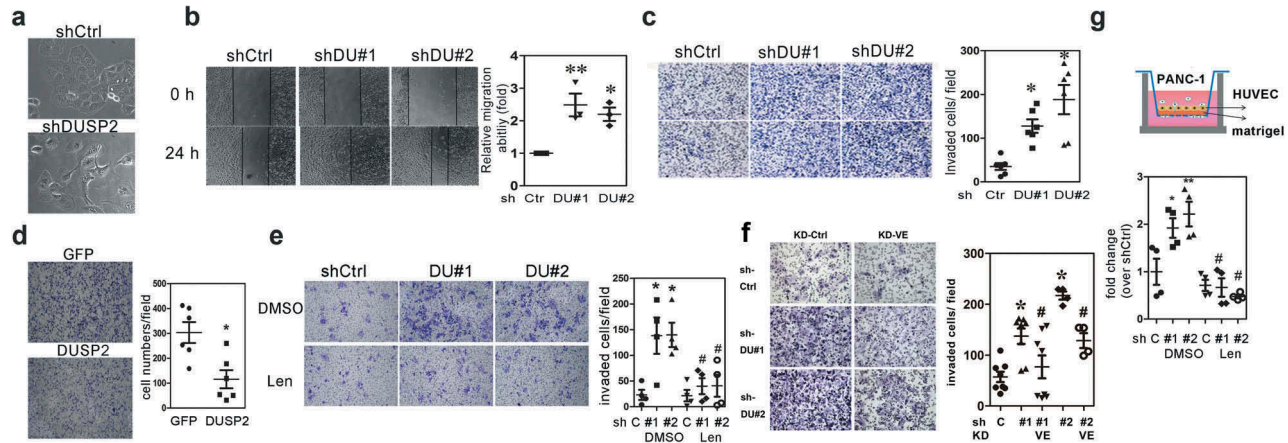
Figure 4. Knockdown of DUSP2 mediates autocrine function in pancreatic cancer cells via VEGF-C signalling. (a) Representative image shows the morphology of control and DUSP2 knockdown in PANC-1 cells. (b) Representative image (left) and the quantitative result (right, n = 3 ) show the migration ability in DUSP2-KD PANC-1 cells. Control (ctrl) and DUSP2-KD (DU#1 and DU#2) PANC-1 cells were seeded in the 24-well plate to confluent and a straight scratch was made by pipette tips. Images were recorded and analysed after 24 h. (c) Representative image (left) and the quantitative result (right, n = 3 ) show cell invasion ability in control and DUSP2-KD PANC-1 cells. (d) Expression of DUSP2-GFP in MIA PaCa-2 cells inhibited cell migration through transwell. MIA PaCa-2 cells were transfected with GFP or DUSP2-GFP, equal numbers of cells were plated on top of transwell. Data represent mean and SEM from two independent experiments (performed in triplicate) using different batches of cells. (e) Representative images (left) and the quantitative result (right, n = 3 ) show increased invasion ability in DUSP2-KD PANC-1 cells was suppressed when treated with VEGFR2/R3 inhibitor, Lenvatinib (10 nM). *P < 0.05 compared to control, \#P < 0.05 compared to DUSP2-KD. (f) Representative images (left panels) and quantitative result (right, n = 3 ) show knockdown of VEGF-C abolished loss-of-DUSP2-mediated increased invasion ability. VEGF-C was transiently knocked down in control and DUSP2-KD PANC-1 cells. Cell invasion ability was measured in matrigel-coated transwell. *P < 0.05 compared to control, \#P < 0.05 compared to DUSP2-KD. (g) Schematic diagram (top) and quantitative result (bottom, n = 3 ) show increased transendothelial migration assay in control and DUSP2-KD PANC-1 cells were suppressed when treated with VEGFR2/R3 inhibitor. Endothelial cells were seeded to a matrigel-coated transwell. After the endothelial layer was formed, PANC-1 control and DUSP2-KD cells were added to the chamber and transendothelial migration ability was measured after 16 h. *P < 0.05 compared to control, \#P < 0.05 compared to DUSP2-KD. *P < 0.05 ; **P < 0.01 .
